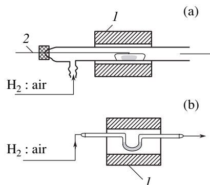
Fig. 1. Schematic of the reactor assembly: (a) cylindrical reactor ( d = 1.8 cm) with a boat for the molybdenite sample, (b) a U-shape reactor ( d = 0.8 cm) filled with molybdenite sample. (1) a heater with a temperature controller, (2) a capillary for gas sampling for chromatographic analysis.
