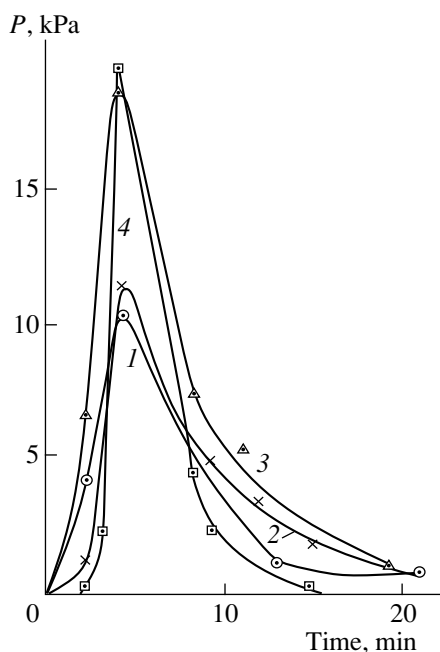
Fig. 2. Kinetics of hydrogen sulfide formation in the reactor (1.8 cm in diameter). P_{H_2} : P_{air} = 3 : 1 . The boat with the following sample was placed into the reactor: (1) the molybdenite sample; (2) the molybdenite sample with rectangular quartz pieces buried in the powder to half-length, (3) the molybdenite sample with horizontal quartz cylinders buried in the powder to 2/3 of the length, and (4) the molybdenite sample with relatively small quartz pieces put onto the sample surface.
